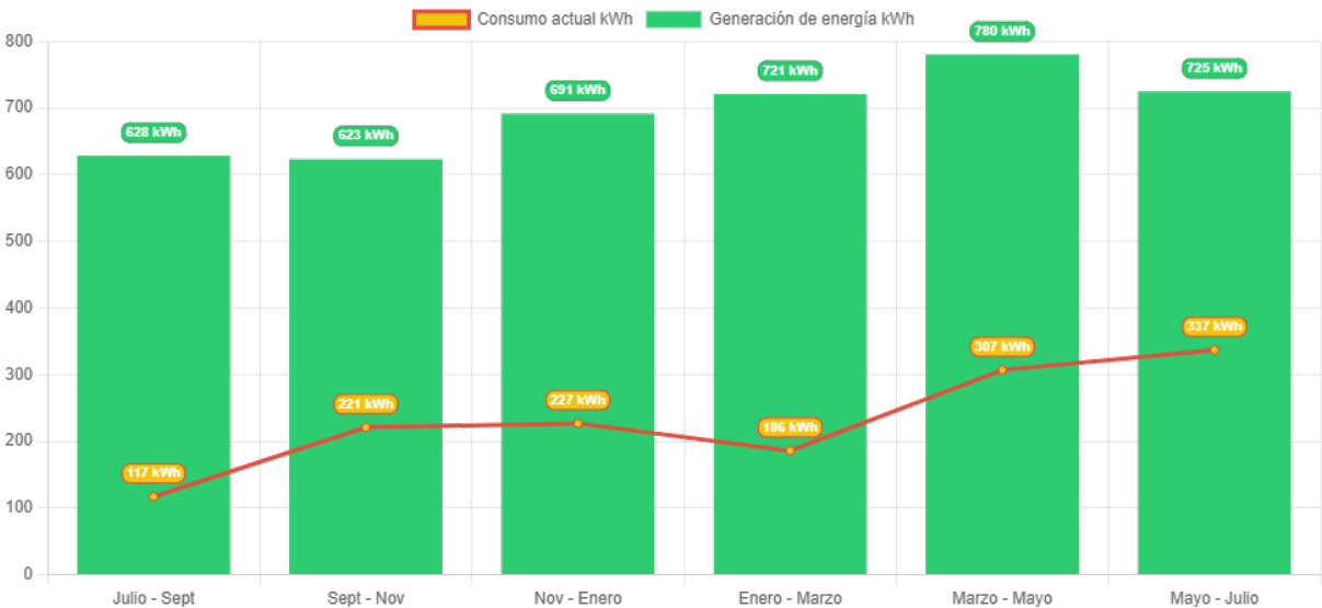
C250910 - SOLAR FV 2.48 kWp (STD)
